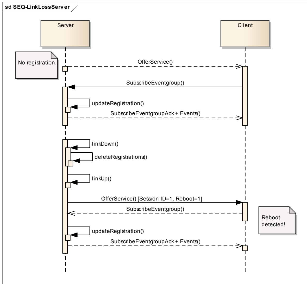
Figure 6.29: Publish/Subscribe with link loss at server (figure ignoring timings)
