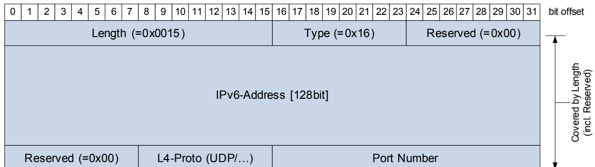
Figure 6.19: SOME/IP-SD IPv6 Multicast Option
