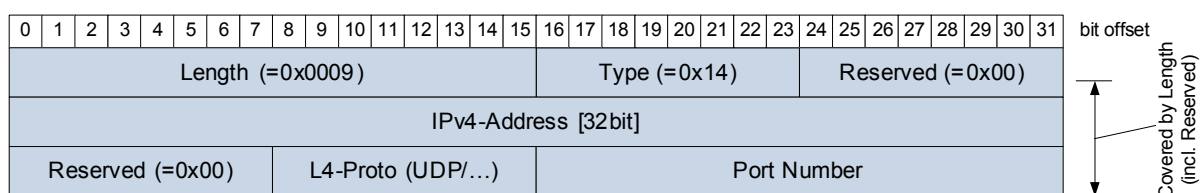
Figure 6.17: SOME/IP-SD IPv4 Multicast Option
