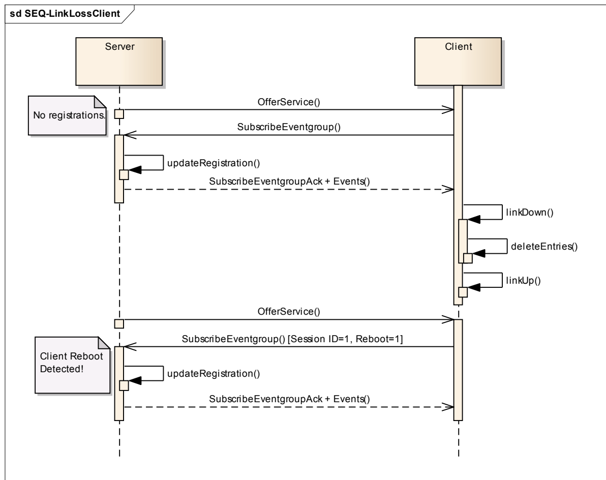
Figure 6.24: Publish/Subscribe with link loss at client (figure ignoring timings)
