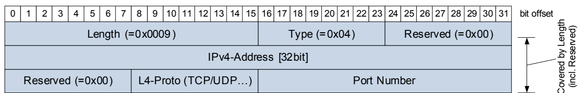
Figure 6.15: SOME/IP-SD IPv4 Endpoint Option
