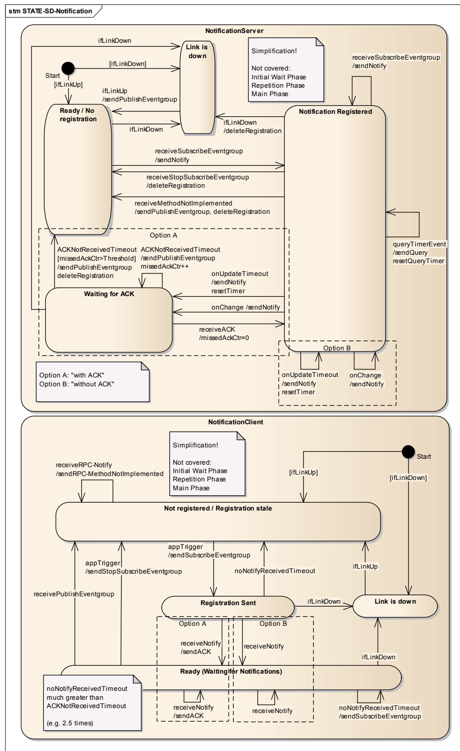
Figure 6.30: Publish/Subscribe State Diagram (overall behavior)
