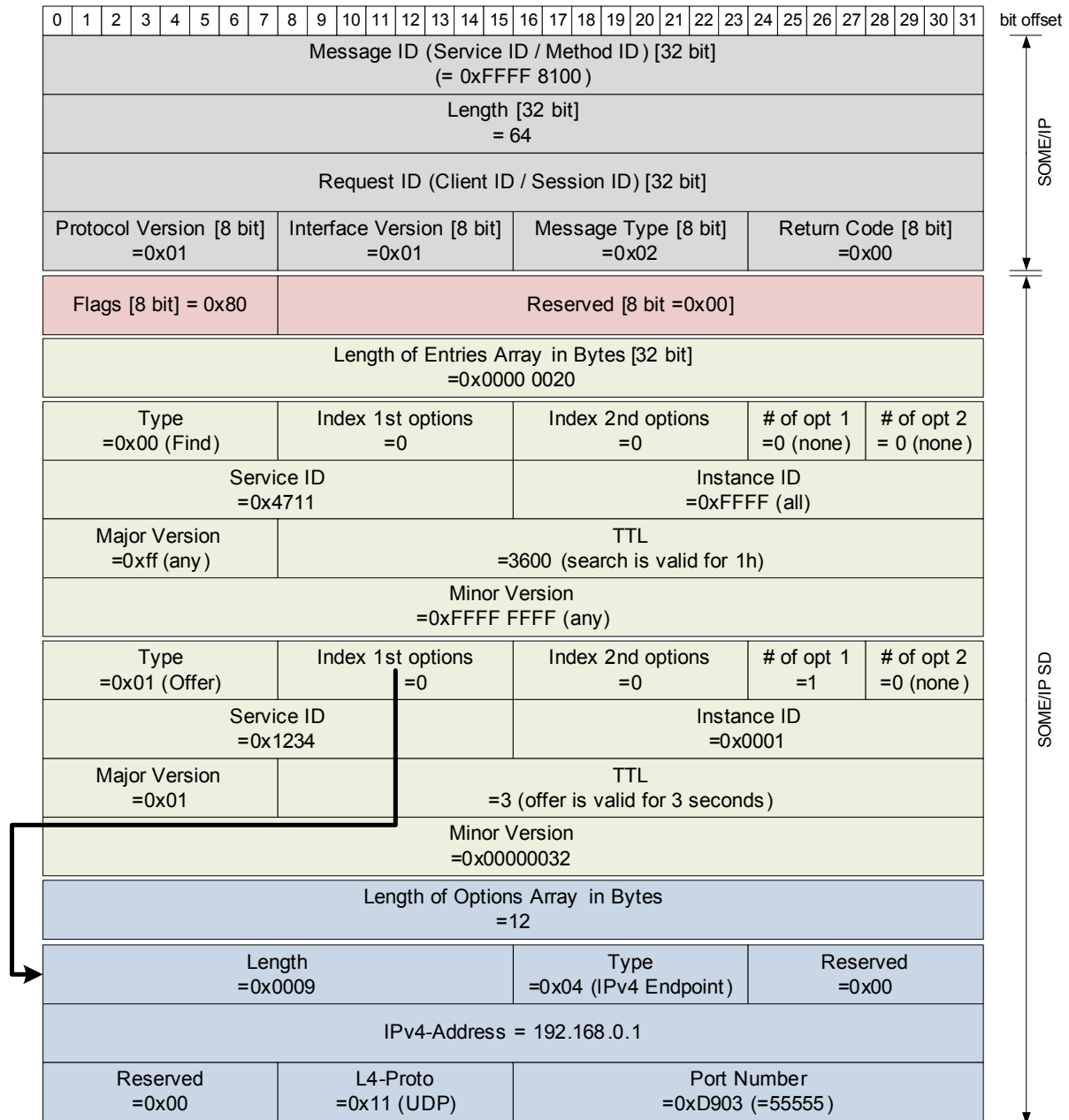
Figure 6.19: SOME/IP-SD Example PDU
