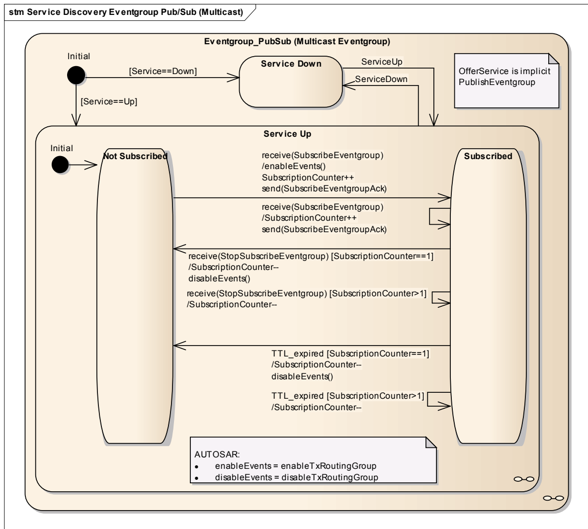
Figure 6.28: Publish/Subscribe State Diagram (server behavior for multicast eventgroups)
