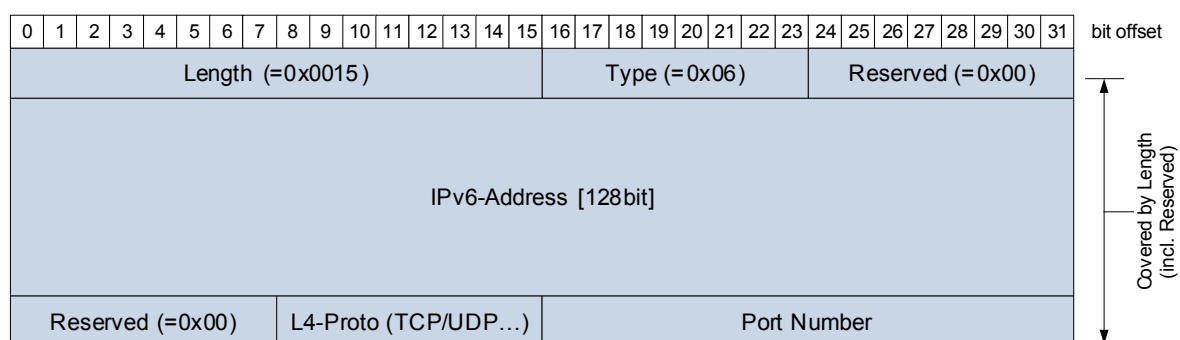
Figure 6.16: SOME/IP-SD IPv6 Endpoint Option
