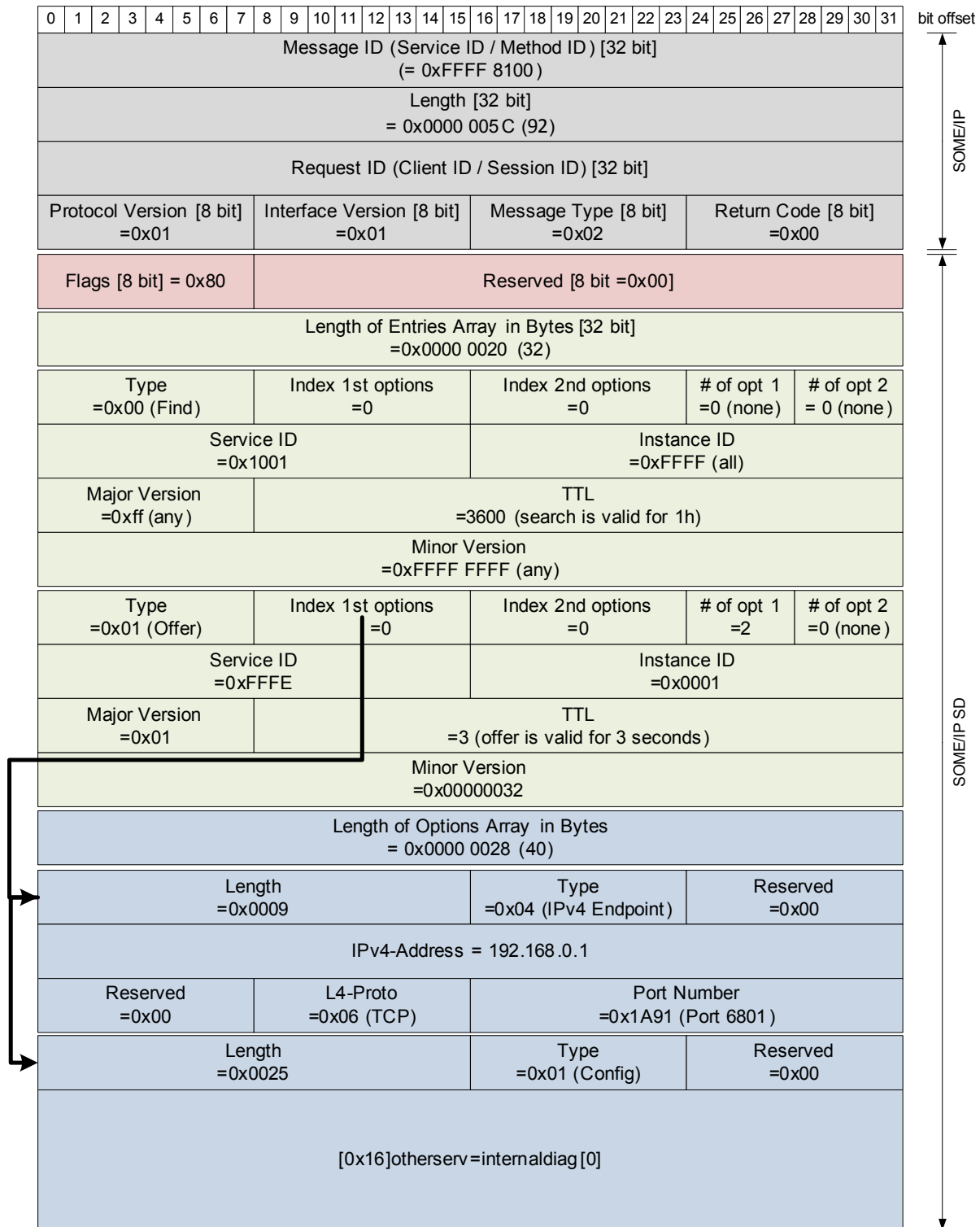
Figure 6.22: SOME/IP-SD Example PDU for Non-SOME/IP-SD
