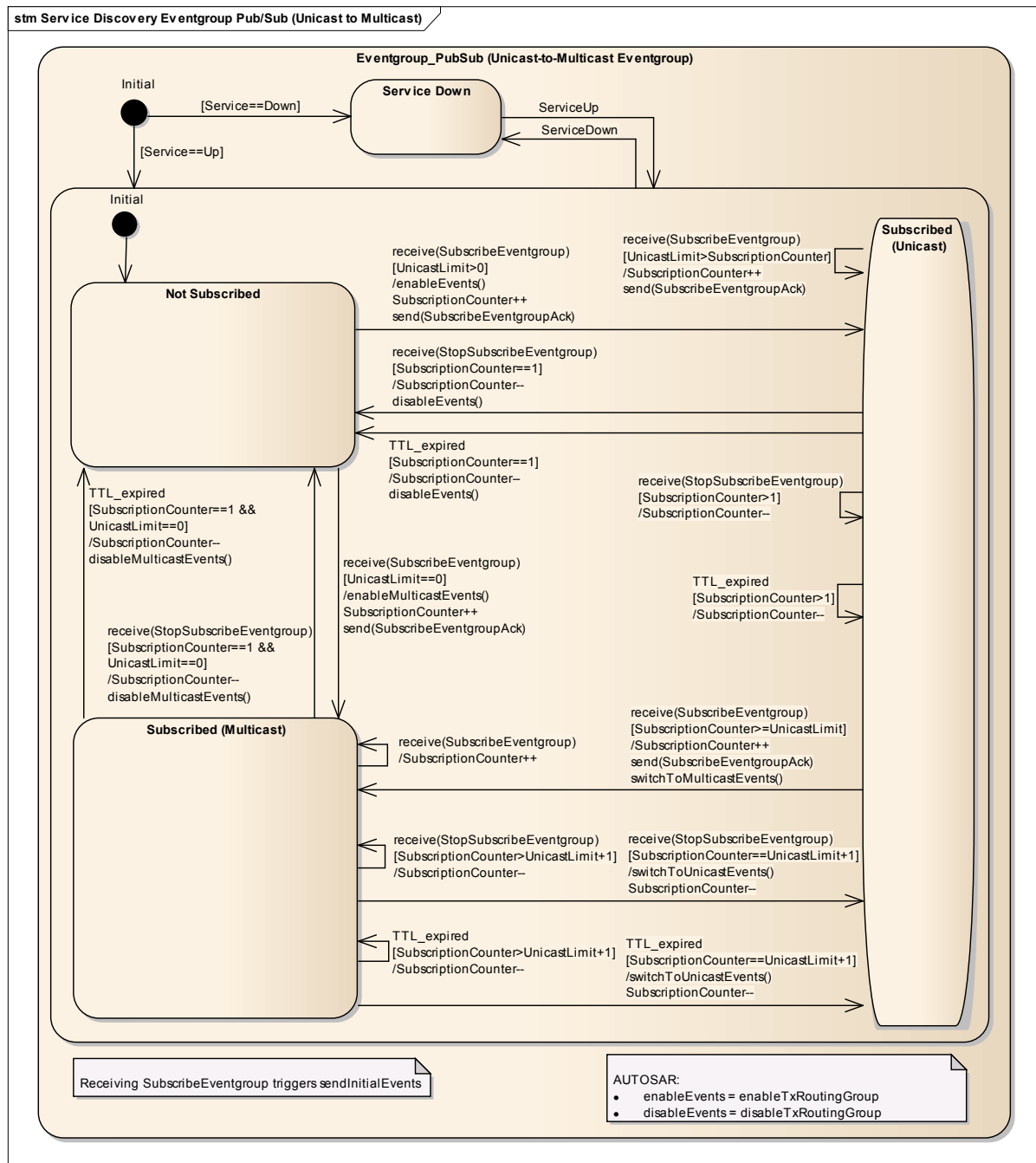
Figure 6.29: Publish/Subscribe State Diagram (server behavior for adaptive unicast/multicast eventgroups)
