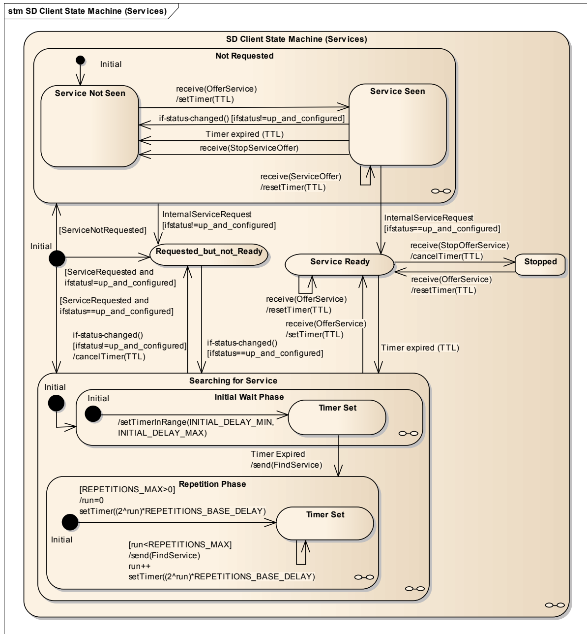
Figure 6.21: SOME/IP Service State Machine Client
