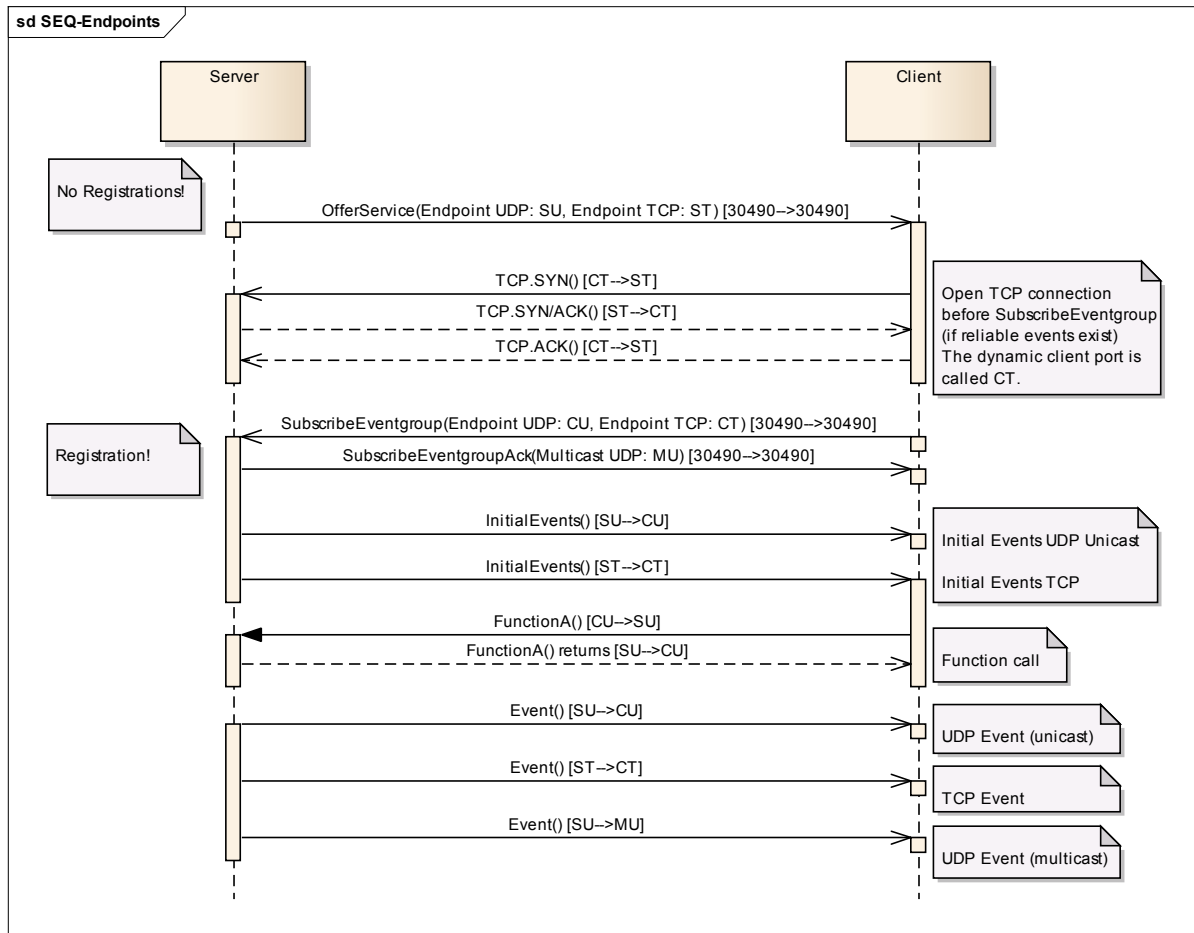
Figure 6.31: Publish/Subscribe Example for Endpoint Options and the usage of ports
