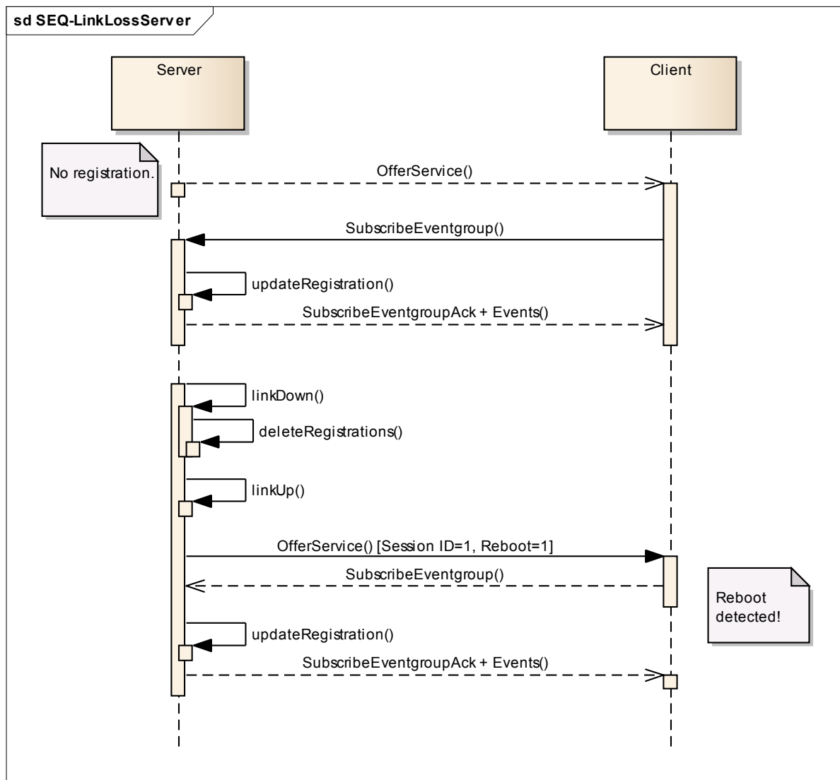
Figure 6.26: Publish/Subscribe with link loss at server (figure ignoring timings)
