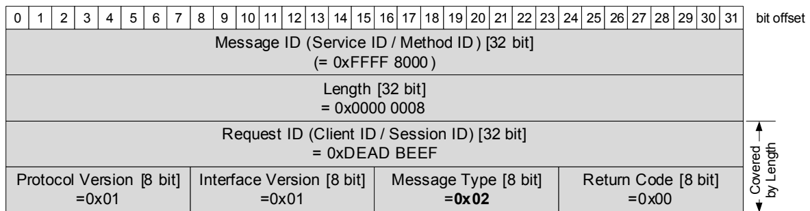
Figure 6.7: SOME/IP Magic Cookie Message for SOME/IP
