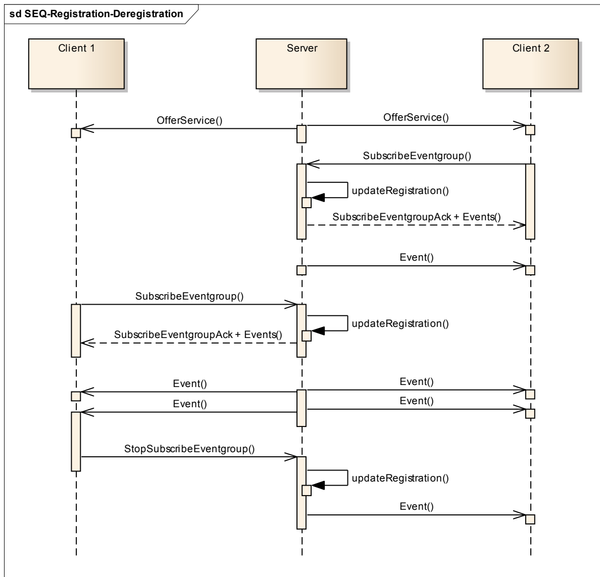
Figure 6.25: Publish/Subscribe Registration/Deregistration behavior (figure ignoring timings)
