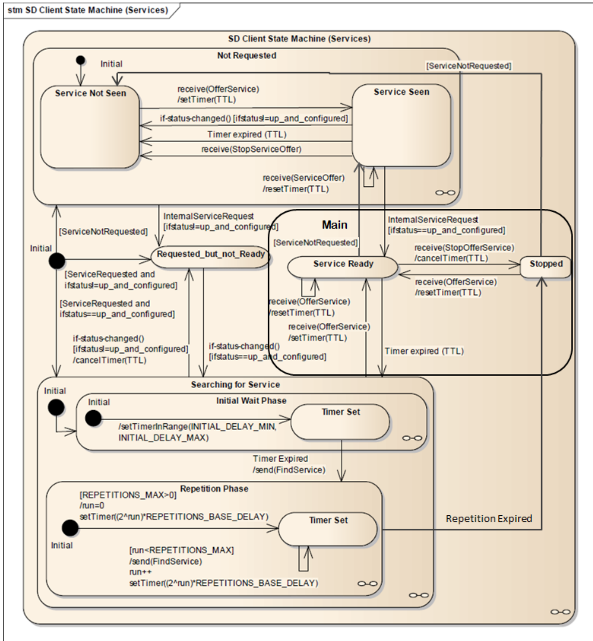
Figure 4.16: SOME/IP Service State Machine Client
