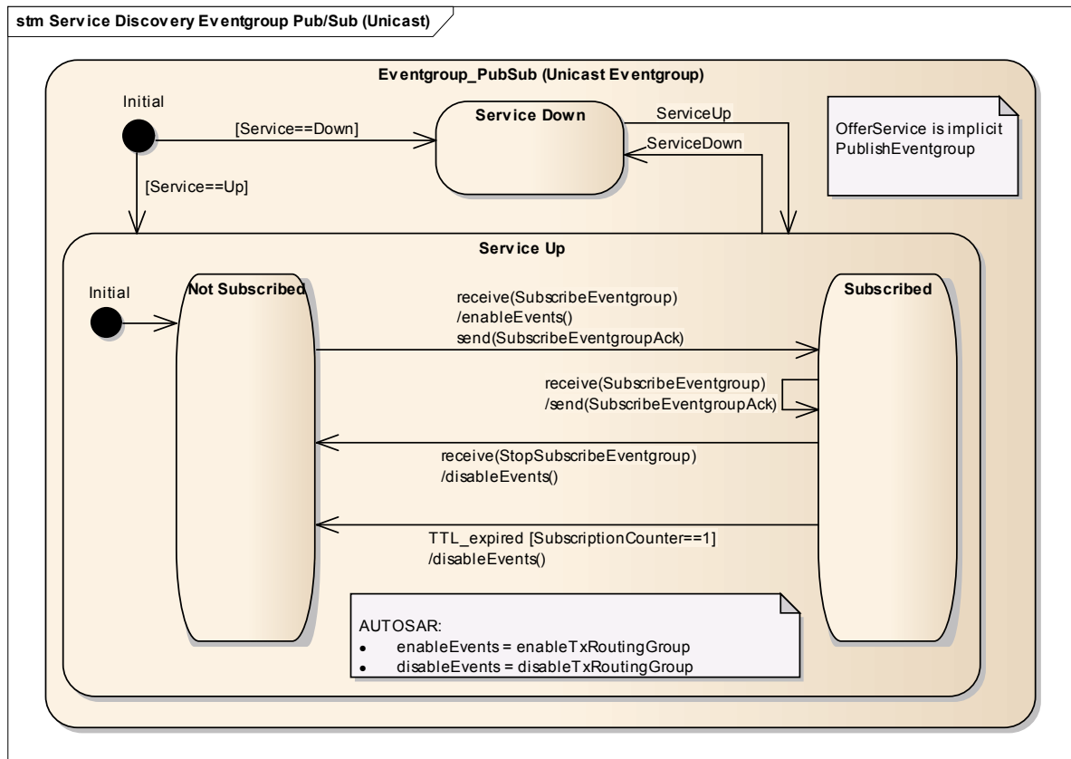
Figure 4.23: Publish/Subscribe State Diagram (server behavior for unicast eventgroups)
