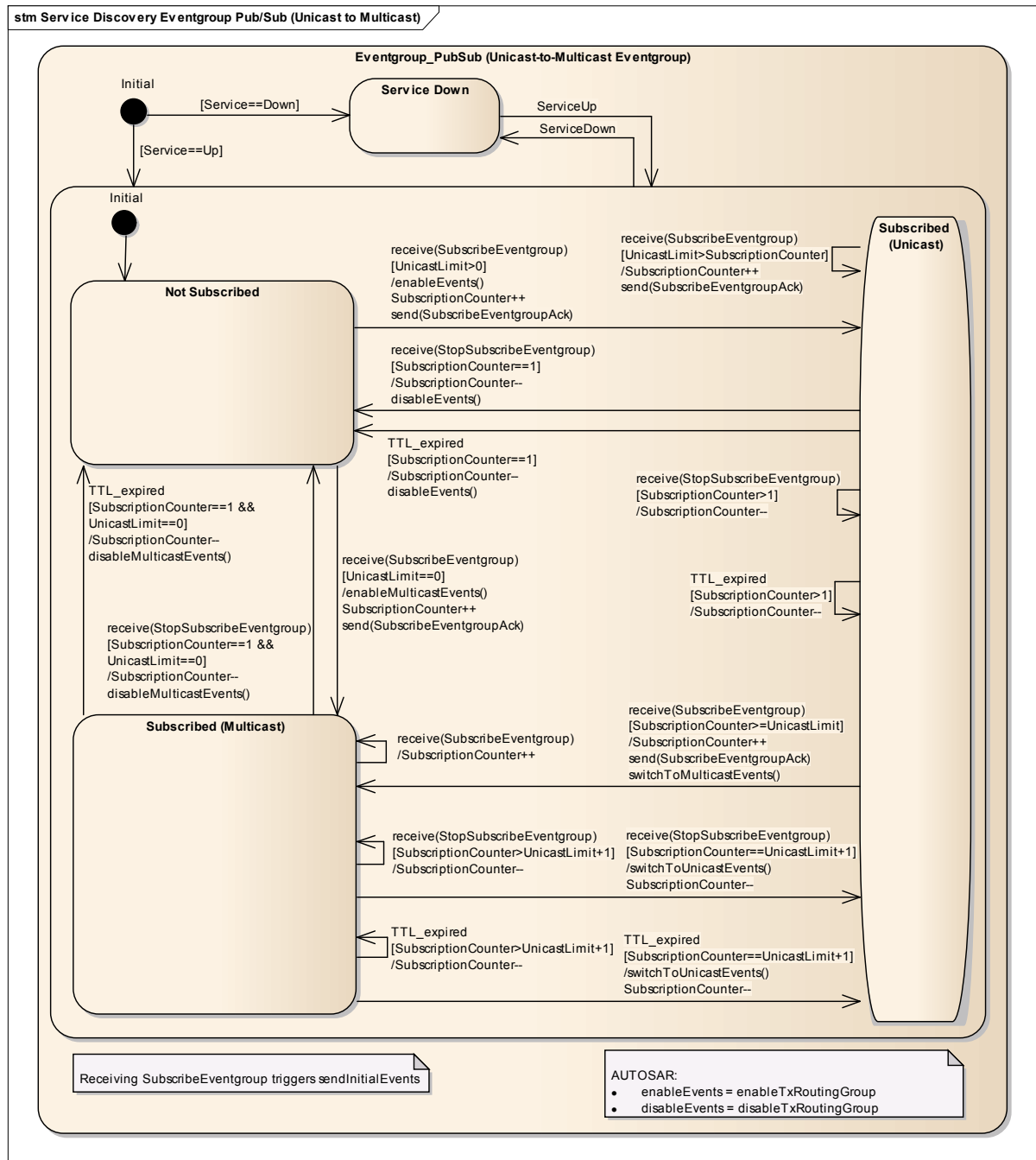
Figure 4.25: Publish/Subscribe State Diagram (server behavior for adaptive unicast/multicast eventgroups)
