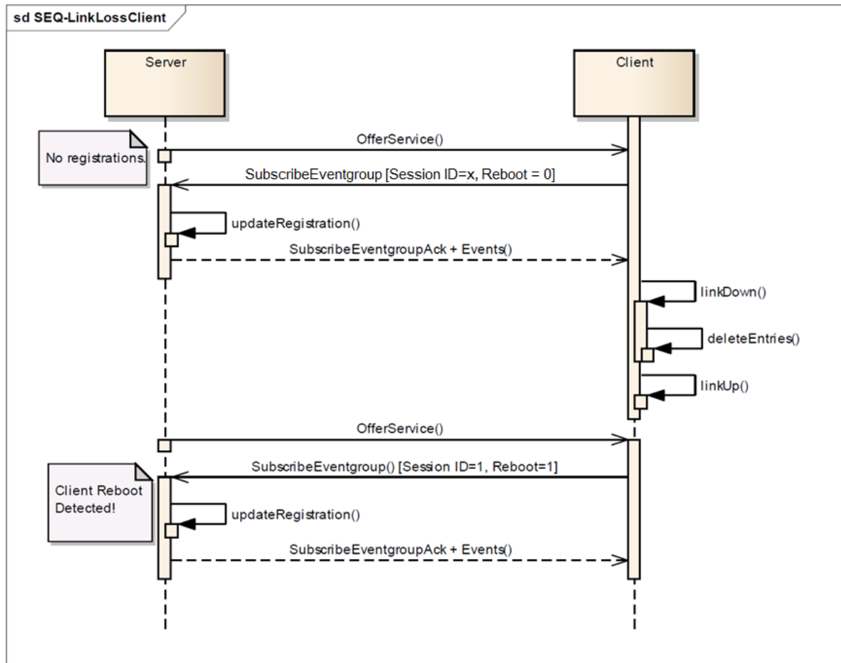
Figure 4.20: Publish/Subscribe with link loss at client (figure ignoring timings)
