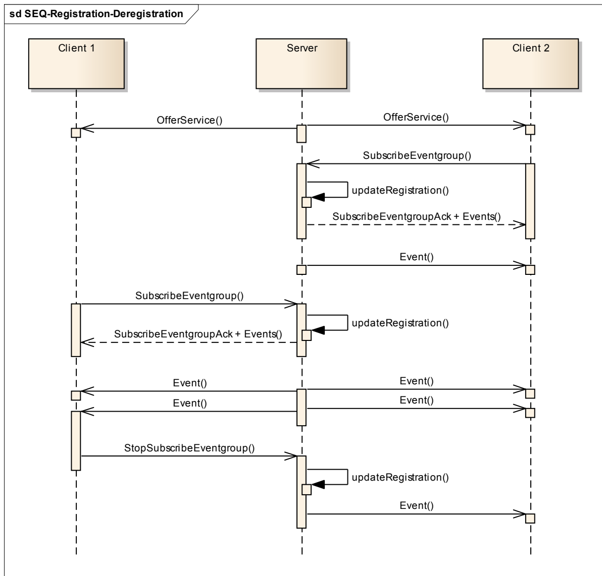
Figure 4.21: Publish/Subscribe Registration/Deregistration behavior (figure ignoring timings)
