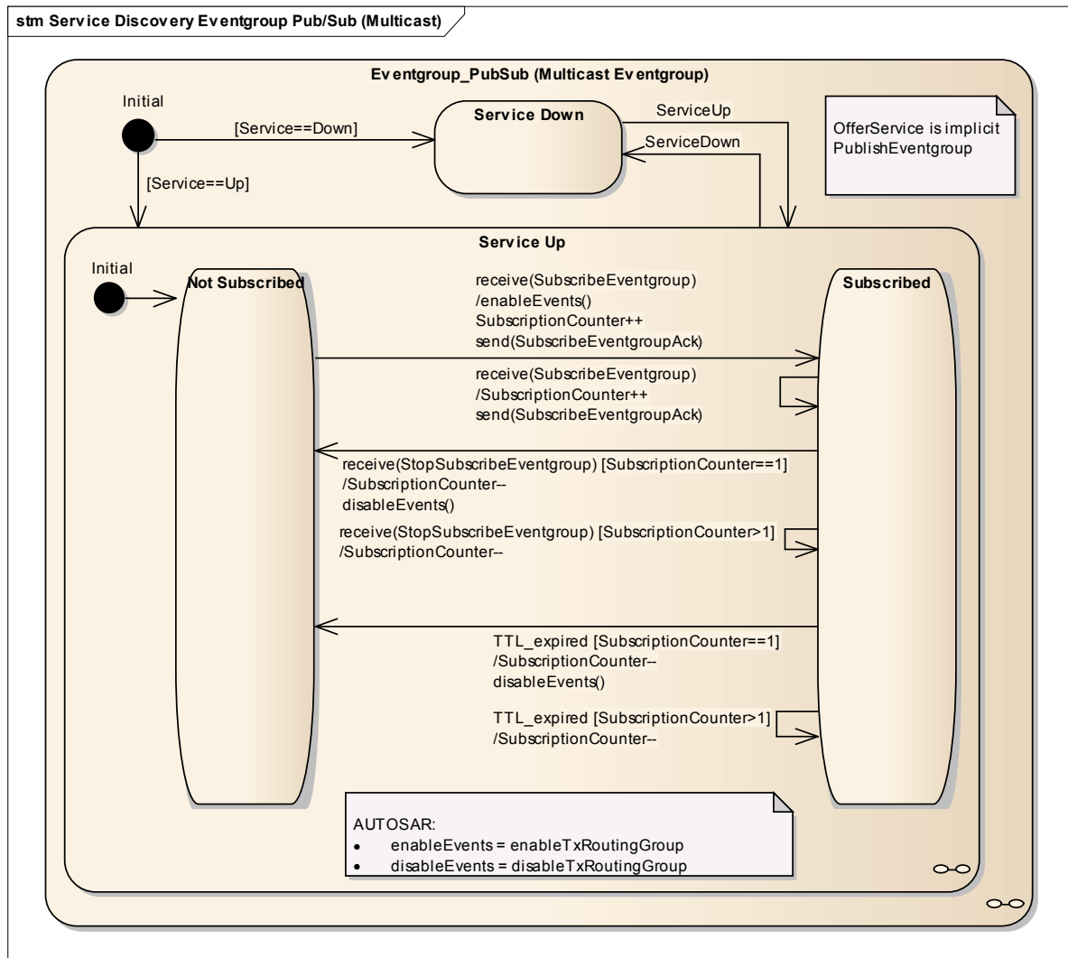
Figure 4.24: Publish/Subscribe State Diagram (server behavior for multicast eventgroups)
