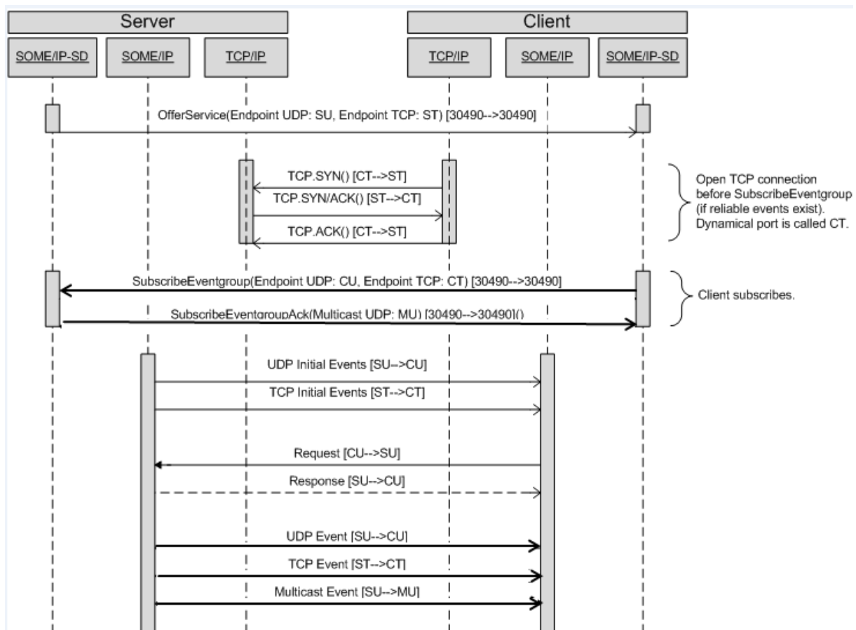
Figure 4.26: Publish/Subscribe Example for Endpoint Options and the usage of ports
