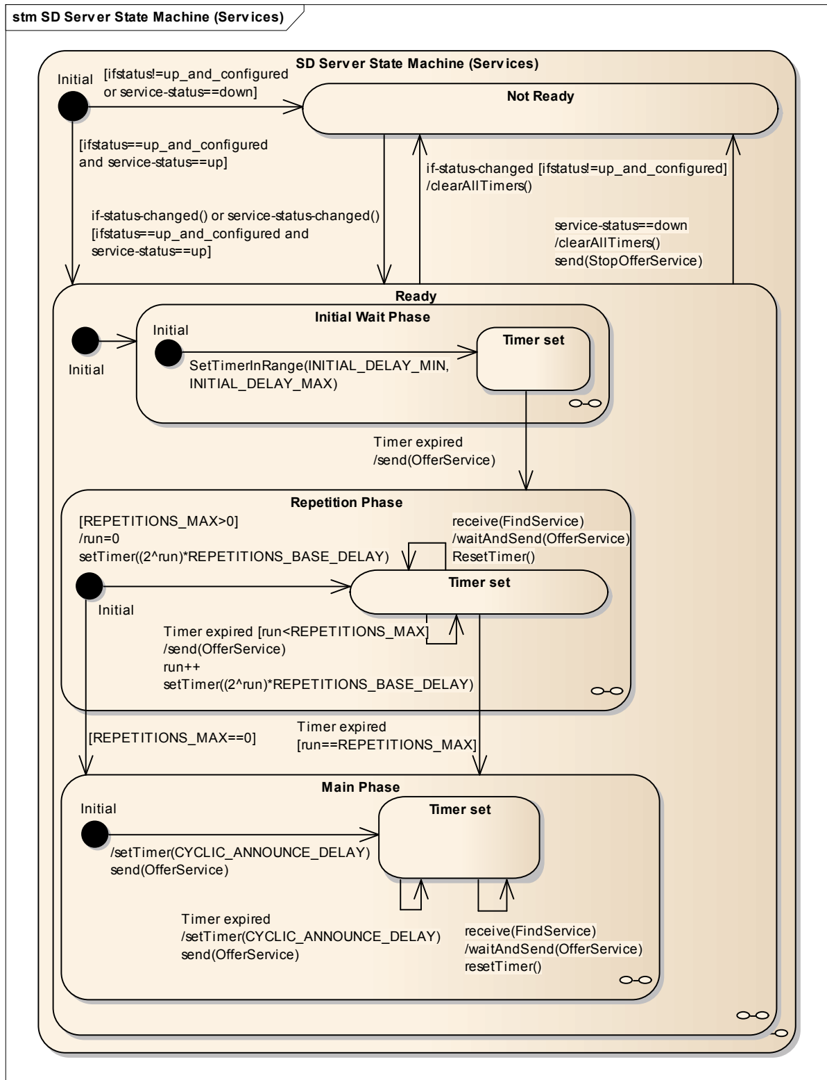
Figure 4.15: SOME/IP Service State Machine Server
