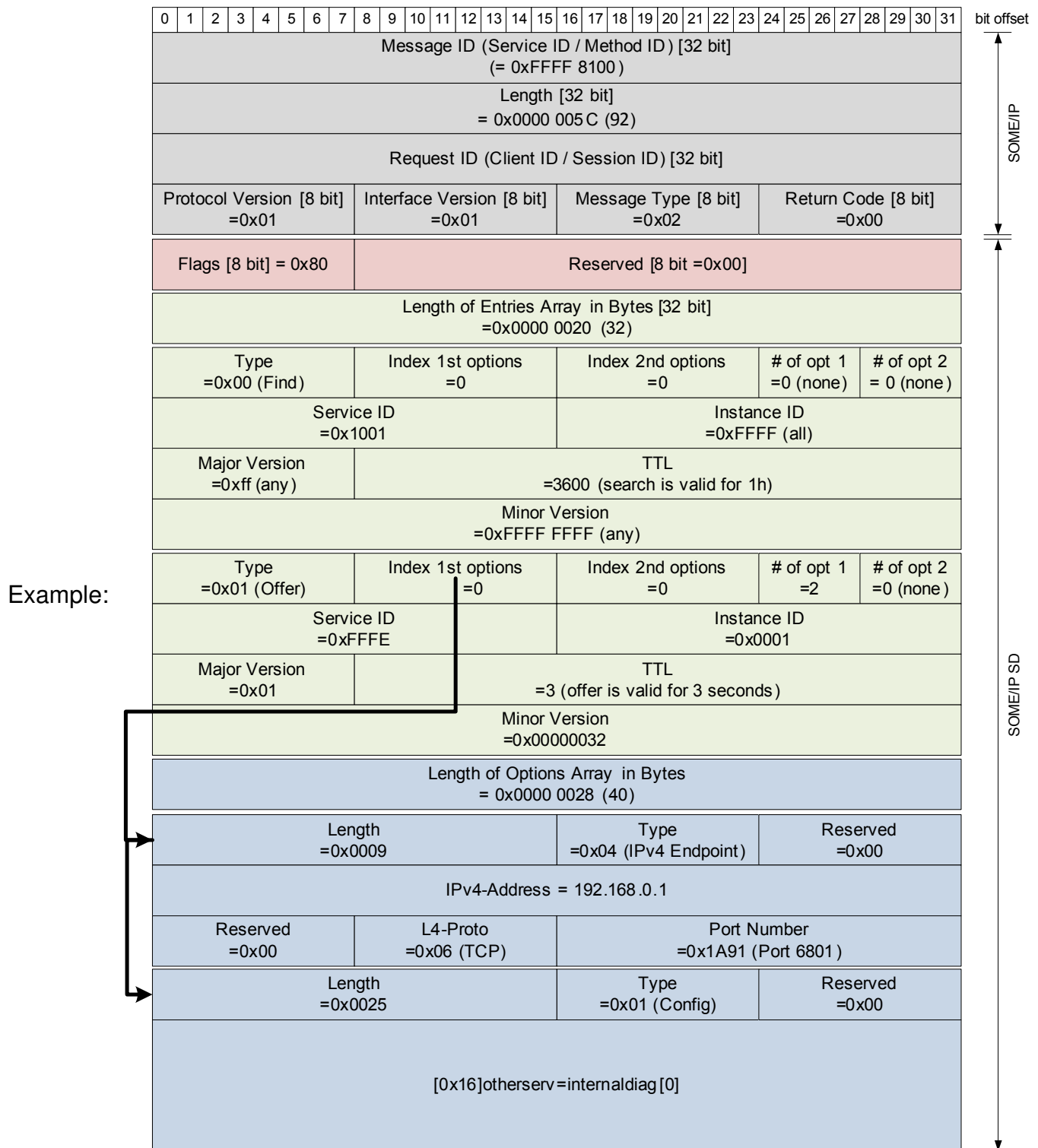
Figure 4.18: SOME/IP-SD Example PDU for Non-SOME/IP-SD
